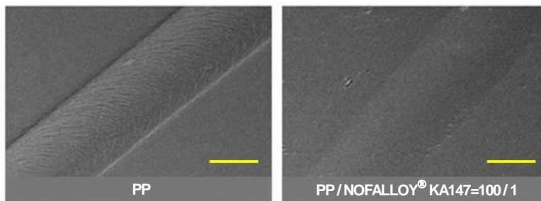
Fig.1 SEM images of PP surface after Scratch test(scale bar: 100μm)
